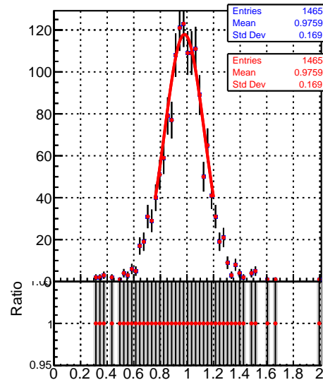
Jet response (pT/pTgen) in 49 <= pt < 64, 3.0 <= |eta| < 5.0
