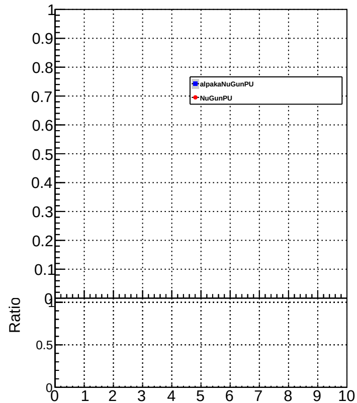
muonMultiplicity
