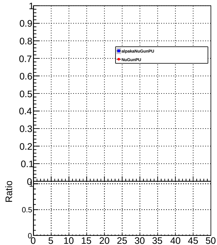
neutralHadronMultiplicity
