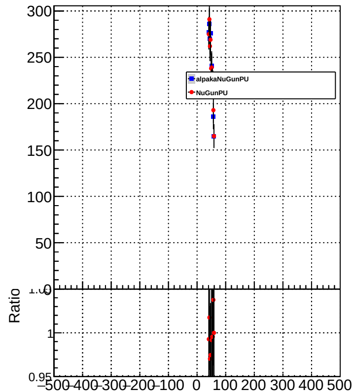
METResolution_GenMETTrue_MET40to60
