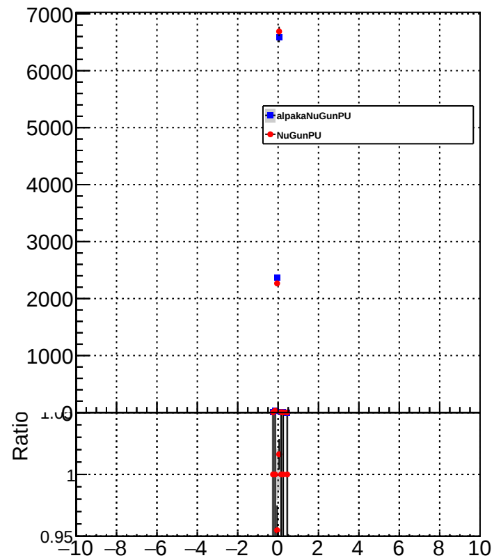
METUnc_ElectronEnUp
