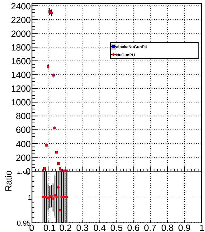
neutralHadronEtFraction
