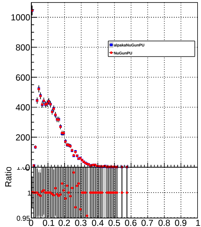
HFHadronEtFraction
