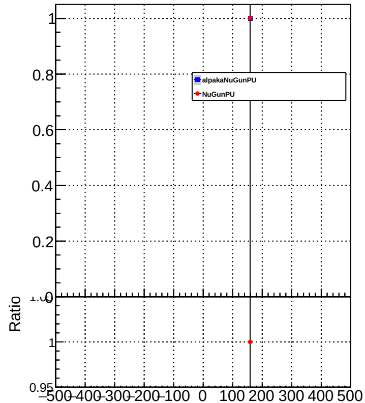
METResolution_GenMETTrue_MET150to200
