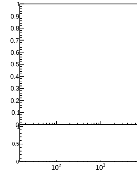
Jet pT response, 0.5 < |\eta| < 1.3
