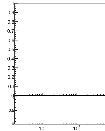
Jet pT response, 2.1 < |\eta| < 2.5
