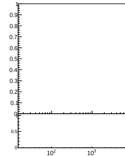
Jet pT response, 2.5 < |\eta| < 3.0
