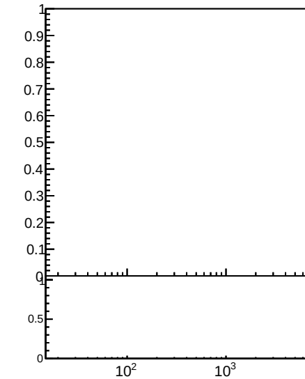
Jet pT response, 1.3 < |\eta| < 2.1
