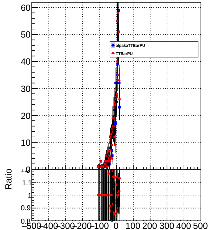
METResolution_GenMETTrue_MET0to20
