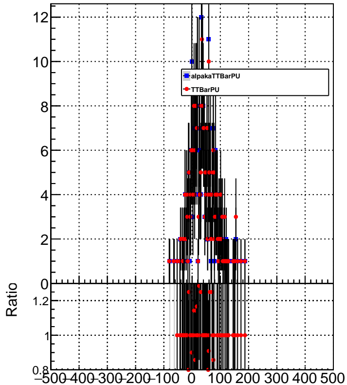
METResolution_GenMETTrue_MET150to200
