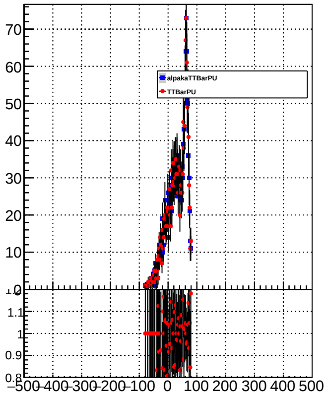
METResolution_GenMETTrue_MET60to80
