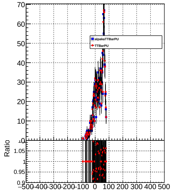
METResolution_GenMETTrue_MET60to80
