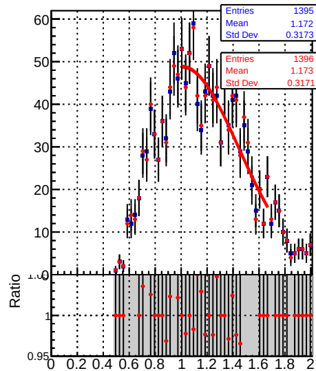
Jet response ( pT/pT_{\text{gen}} ) in 15 \leq pT < 21 , 1.3 \leq |\eta| < 2.1
