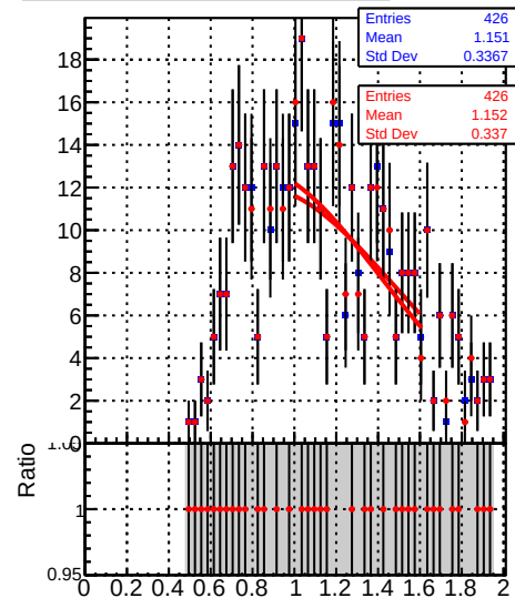
Jet response ( pT/pT_{\text{gen}} ) in 15 \leq pT < 21 , 2.1 \leq |\eta| < 2.5
