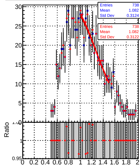
Jet response ( pT/pT_{\text{gen}} ) in 15 \leq pT < 21 , 3.0 \leq |\eta| < 5.0
