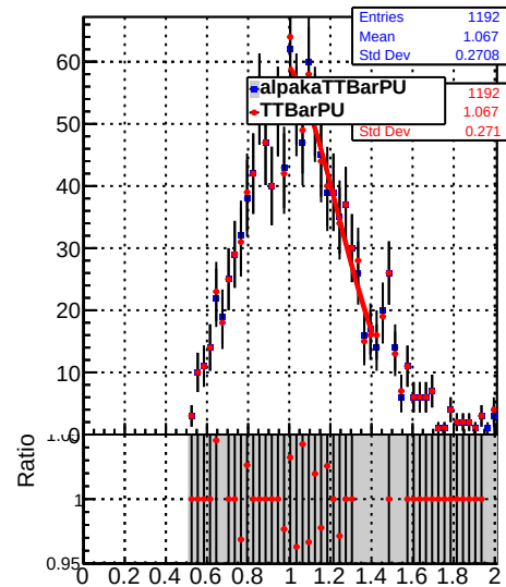
Jet response ( pT/pT_{\text{gen}} ) in 15 \leq pT < 21 , 0.0 \leq |\eta| < 1.3
