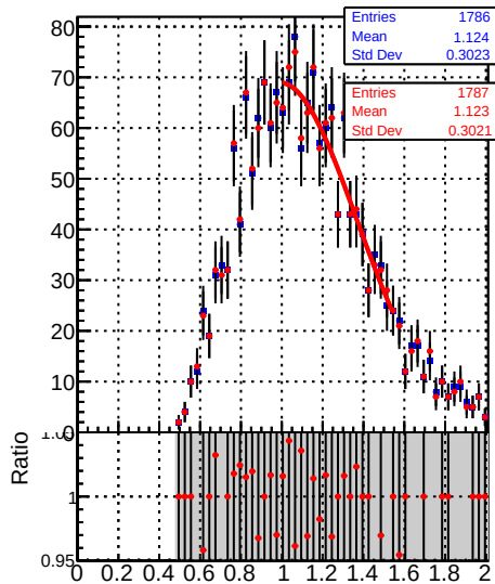
Jet response ( pT/pT_{\text{gen}} ) in 15 \leq pT < 21 , 0.5 \leq |\eta| < 1.3
