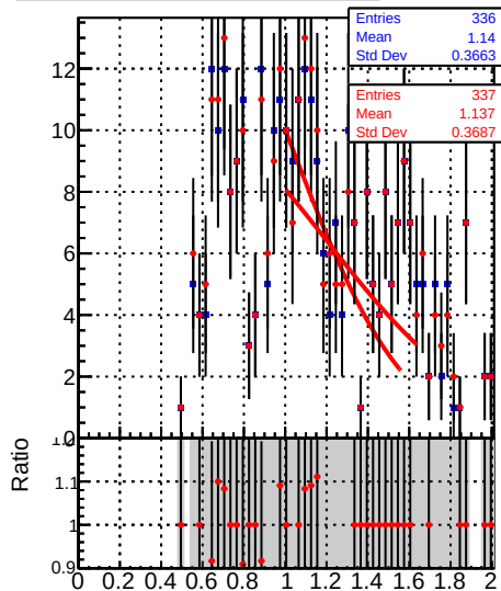
Jet response ( pT/pT_{\text{gen}} ) in 15 \leq pT < 21 , 2.5 \leq |\eta| < 3.0
