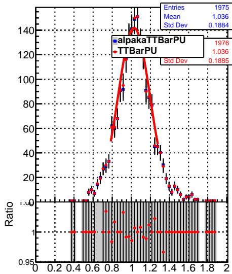
Jet response (pT/pTgen) in 37 \leq pt < 49, 0.5 \leq |\eta| < 0.5
