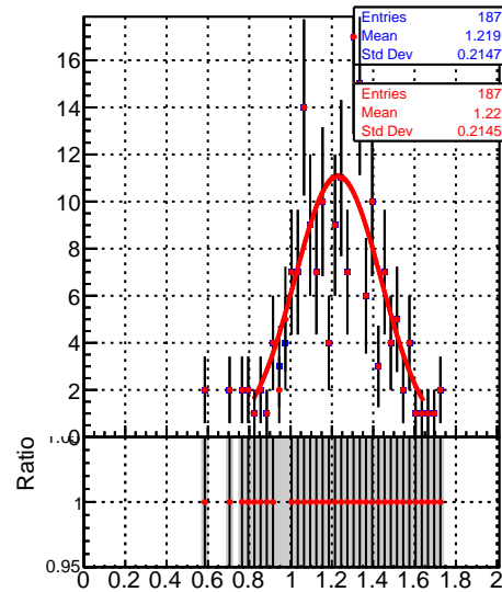
Raw Jet response (pT/pTgen) in 64 &lt;= pt &lt; 84, 3.0 &lt;= |eta| &lt; 5.0
