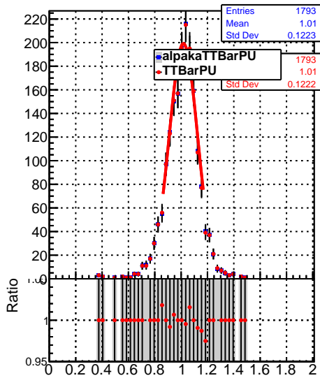
Raw Jet response (pT/pTgen) in 84 &lt;= pt &lt; 114, 0.0 &lt;= |eta| &lt; 0.5
