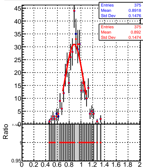
Raw Jet response (pT/pTgen) in 84 &lt;= pt &lt; 114, 2.1 &lt;= |eta| &lt; 2.5
