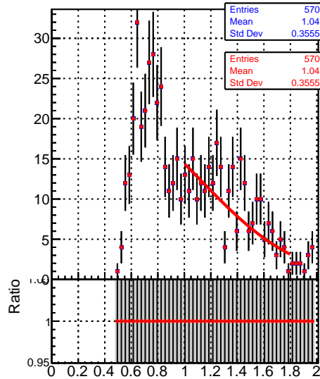
Jet response (pT/pTgen) in 15 \leq p_t < 21, 3.0 \leq |\eta| < 5.0
