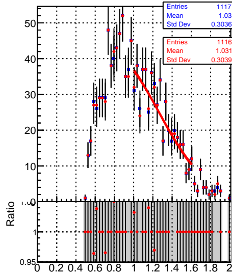
Jet response (pT/pTgen) in 15 \leq p_t < 21, 1.3 \leq |\eta| < 2.1
