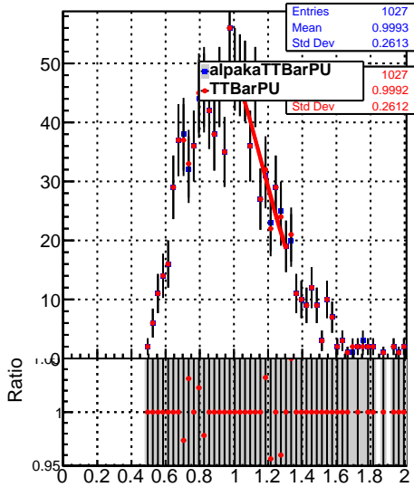
Jet response (pT/pTgen) in 15 \leq p_t < 21, 0.0 \leq |\eta| < 0.5
