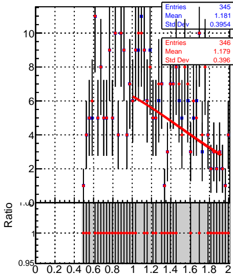
Jet response (pT/pTgen) in 15 \leq p_t < 21, 2.5 \leq |\eta| < 3.0
