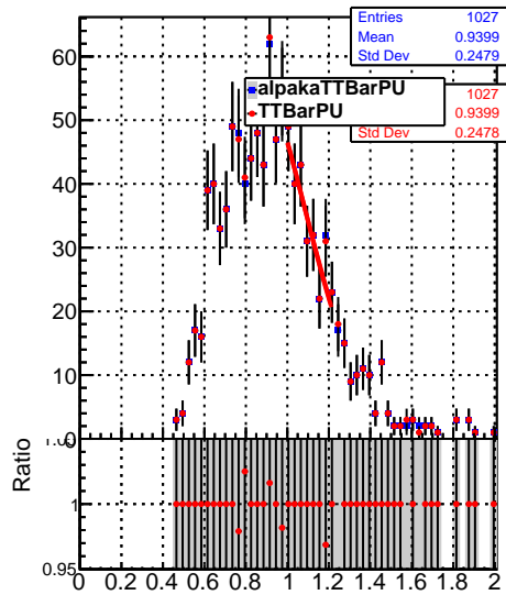
Raw Jet response (pT/pTgen) in 15 &lt;= pt &lt; 21, 0.0 &lt;= |eta| &lt; 0.5
