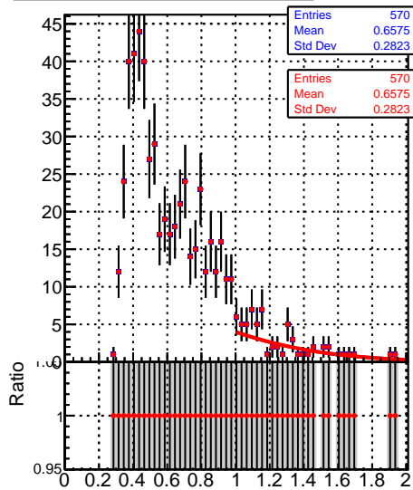
Raw Jet response (pT/pTgen) in 15 &lt;= pt &lt; 21, 3.0 &lt;= |eta| &lt; 5.0
