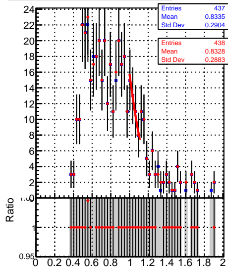
Raw Jet response (pT/pTgen) in 15 &lt;= pt &lt; 21, 2.1 &lt;= |eta| &lt; 2.5
