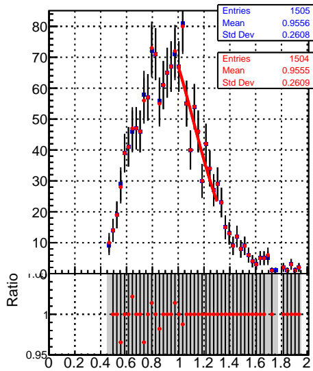
Raw Jet response (pT/pTgen) in 15 &lt;= pt &lt; 21, 0.5 &lt;= |eta| &lt; 1.3
