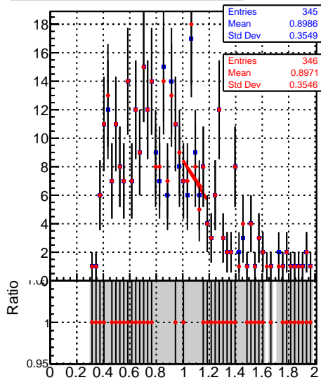
Raw Jet response (pT/pTgen) in 15 &lt;= pt &lt; 21, 2.5 &lt;= |eta| &lt; 3.0
