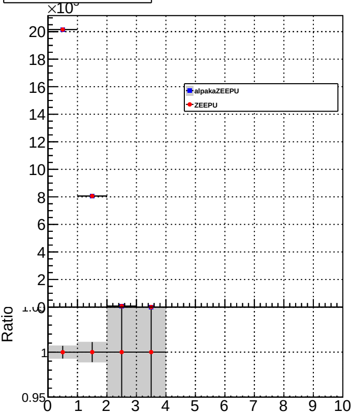
electronMultiplicity
