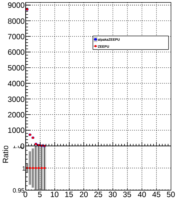
HFHadronMultiplicity
