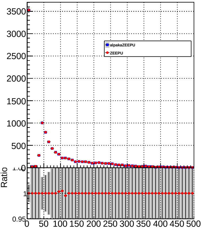
electronEnergy
