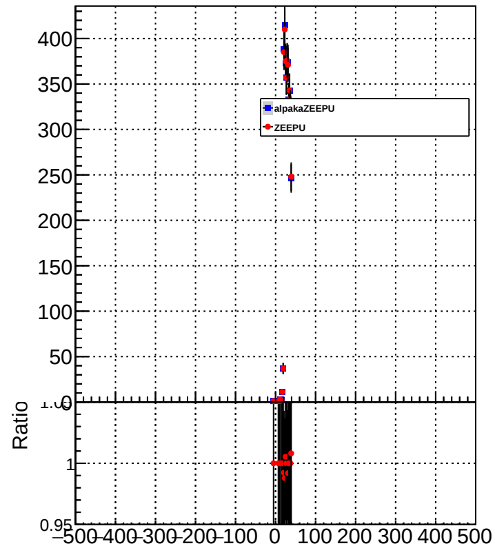
METResolution_GenMETTrue_MET20to40
