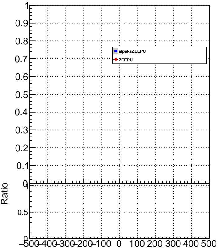
METResolution_GenMETTrue_MET400to500
