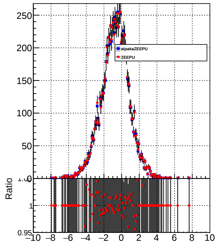
METUnc_UnclusteredEnUp
