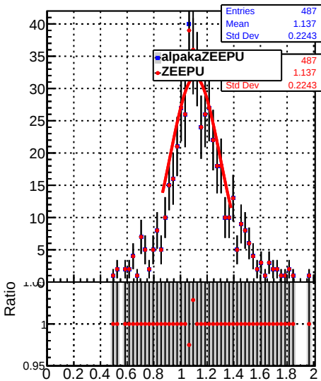
Jet response (pT/pTgen) in 21 \leq p_t < 28, 0.0 \leq |\eta| < 0.5
