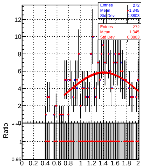
Jet response (pT/pTgen) in 21 \leq p_t < 28, 2.5 \leq |\eta| < 3.0
