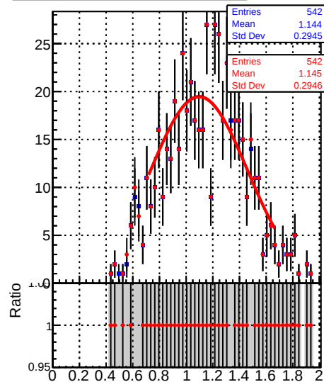
Jet response (pT/pTgen) in 21 \leq p_t < 28, 3.0 \leq |\eta| < 5.0
