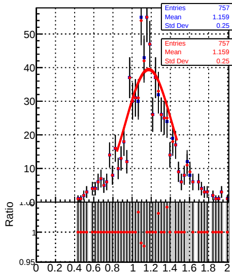
Jet response (pT/pTgen) in 21 \leq p_t < 28, 0.5 \leq |\eta| < 1.3
