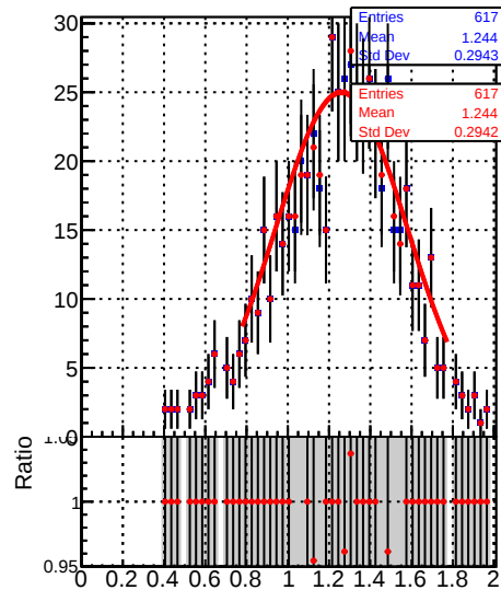
Jet response (pT/pTgen) in 21 \leq p_t < 28, 1.3 \leq |\eta| < 2.1
