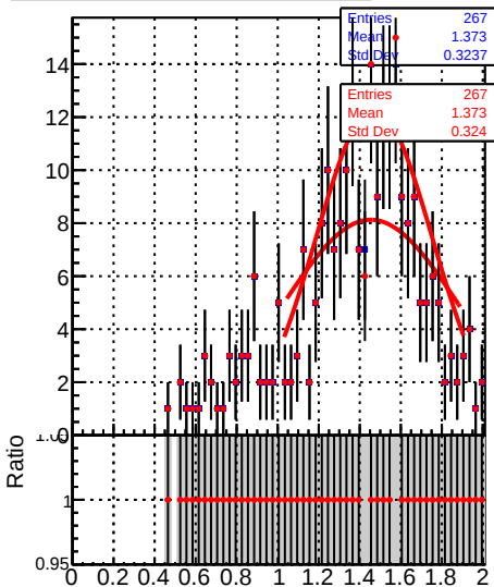
Jet response (pT/pTgen) in 21 \leq p_t < 28, 2.1 \leq |\eta| < 2.5
