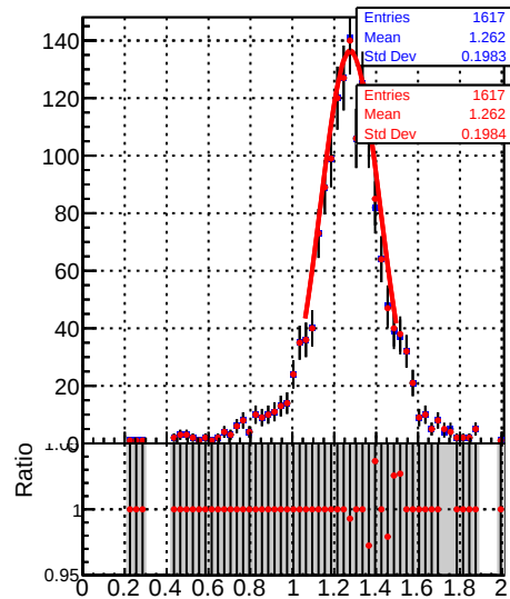
Jet response ( p_T/p_{Tgen} ) in 37 \leq p_T < 49, 1.3 \leq |\eta| < 2.1
