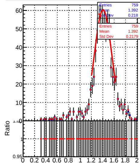
Jet response ( p_T/p_{Tgen} ) in 37 \leq p_T < 49, 2.1 \leq |\eta| < 2.5
