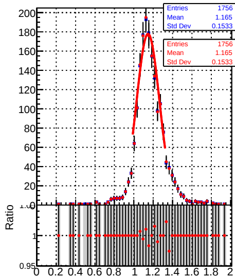
Jet response ( p_T/p_{Tgen} ) in 37 \leq p_T < 49, 0.5 \leq |\eta| < 1.3
