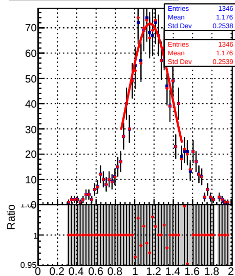
Jet response ( p_T/p_{Tgen} ) in 37 \leq p_T < 49, 3.0 \leq |\eta| < 5.0
