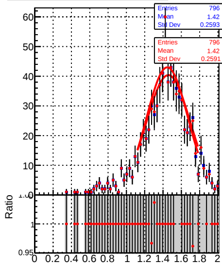
Jet response ( p_T/p_{Tgen} ) in 37 \leq p_T < 49, 2.5 \leq |\eta| < 3.0
