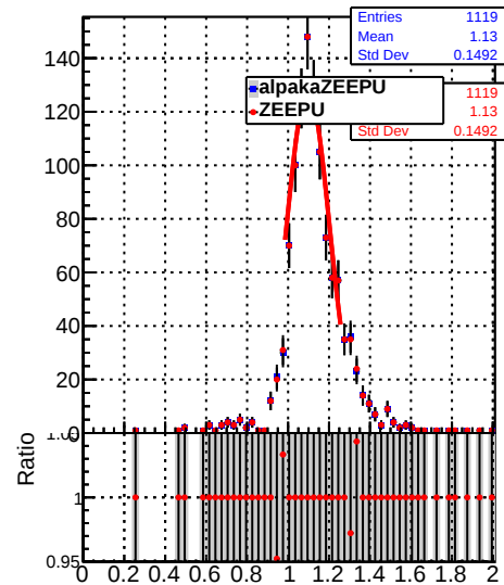
Jet response ( p_T/p_{Tgen} ) in 37 \leq p_T < 49, 0.0 \leq |\eta| < 0.5
