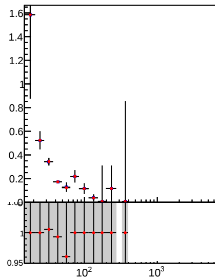
Jet pT resolution, 2.5 < |\eta| < 3.0
