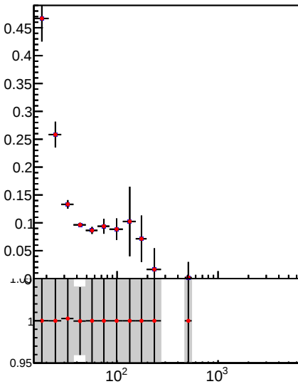
Jet pT resolution, 0.5 < |\eta| < 1.3
