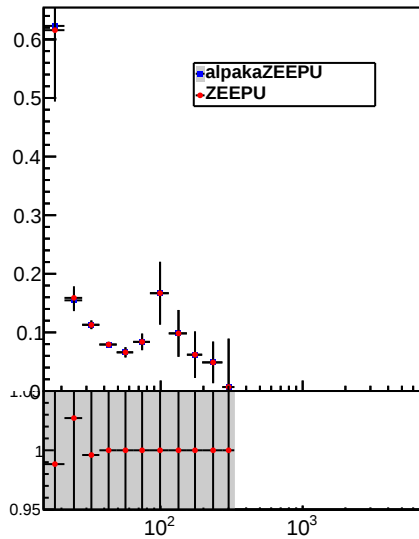
Jet pT resolution, 0.0 < |\eta| < 0.5
