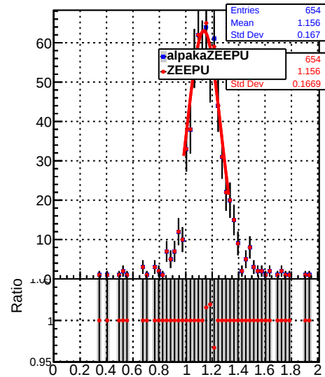
Jet response ( pT/pT_{\text{gen}} ) in 28 \leq pt < 37, 0.0 \leq |\eta| < 0.5
