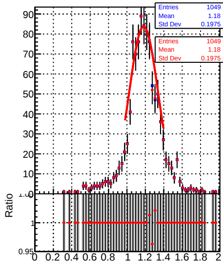
Jet response ( pT/pT_{\text{gen}} ) in 28 \leq pt < 37, 0.5 \leq |\eta| < 1.3
