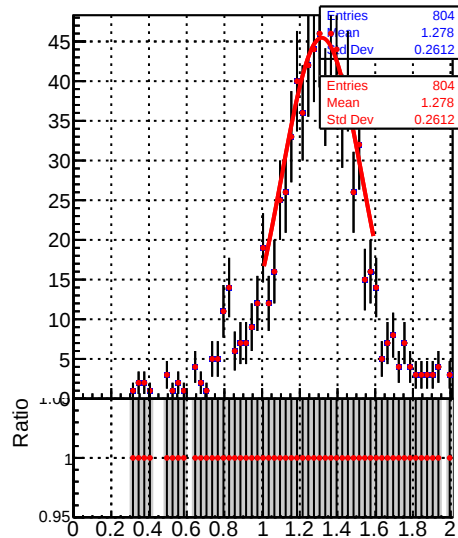
Jet response ( pT/pT_{\text{gen}} ) in 28 \leq pt < 37, 3.0 \leq |\eta| < 5.0
