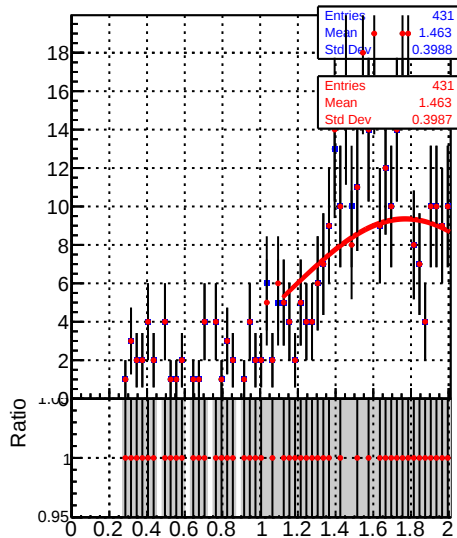
Jet response ( pT/pT_{\text{gen}} ) in 28 \leq pt < 37, 2.5 \leq |\eta| < 3.0
