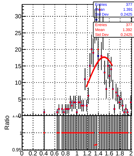
Jet response ( pT/pT_{\text{gen}} ) in 28 \leq pt < 37, 2.1 \leq |\eta| < 2.5
