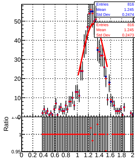
Jet response ( pT/pT_{\text{gen}} ) in 28 \leq pt < 37, 1.3 \leq |\eta| < 2.1
