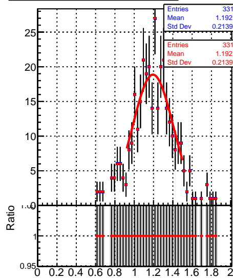
Jet response (pT/pTgen) in 49 \leq pt < 64, 3.0 \leq |\eta| < 5.0
