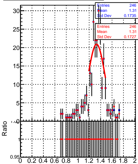
Jet response (pT/pTgen) in 49 \leq pt < 64, 2.1 \leq |\eta| < 2.5
