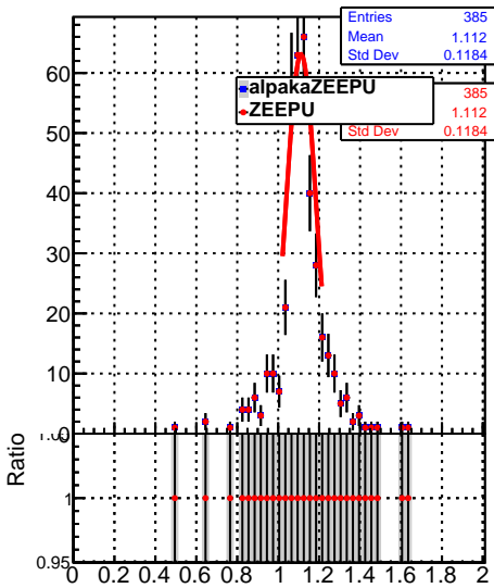
Jet response (pT/pTgen) in 49 \leq pt < 64, 0.0 \leq |\eta| < 0.5
