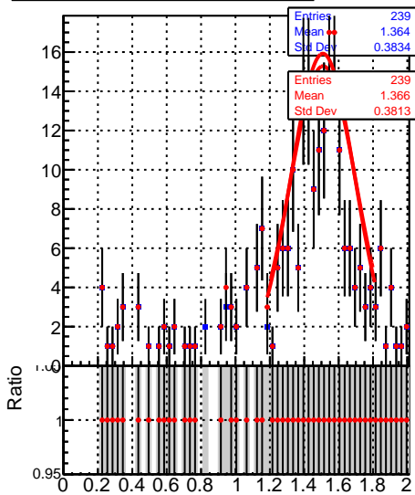
Jet response (pT/pTgen) in 49 \leq pt < 64, 2.5 \leq |\eta| < 3.0
