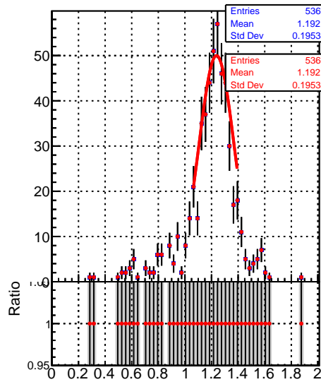
Jet response (pT/pTgen) in 49 \leq pt < 64, 1.3 \leq |\eta| < 2.1
