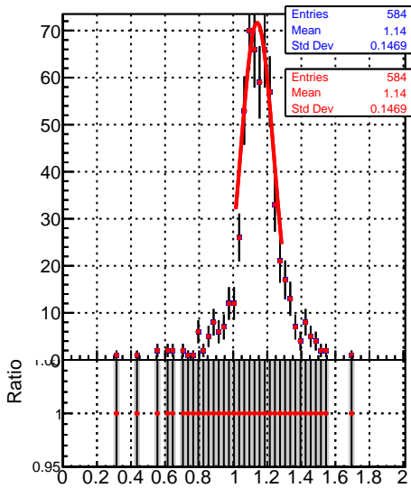
Jet response (pT/pTgen) in 49 \leq pt < 64, 0.5 \leq |\eta| < 1.3
