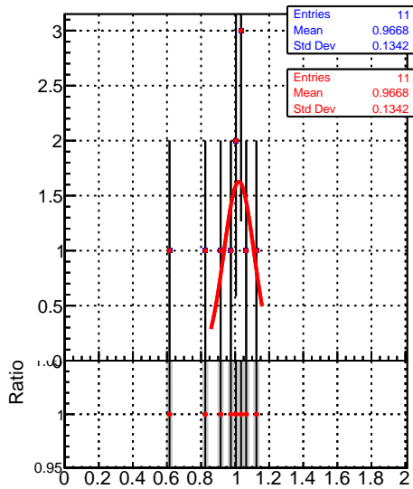
Raw Jet response ( pT/pT_{gen} ) in 153 \leq pt < 196, 0.5 \leq |\eta| < 1.3
