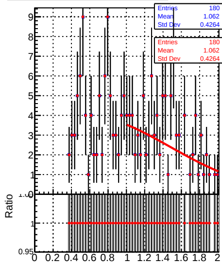
Raw Jet response (pT/pTgen) in 15 \leq p_t < 21, 2.5 \leq |\eta| < 3.0
