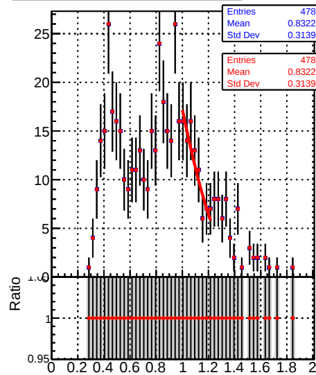
Raw Jet response (pT/pTgen) in 15 \leq p_t < 21, 3.0 \leq |\eta| < 5.0
