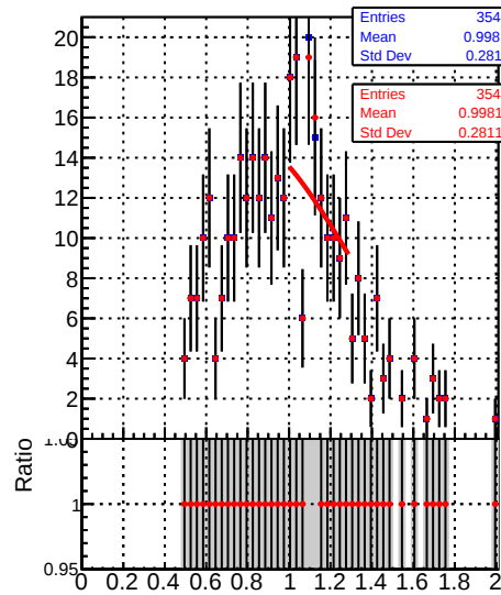
Raw Jet response (pT/pTgen) in 15 \leq p_t < 21, 1.3 \leq |\eta| < 2.1
