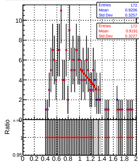
Raw Jet response (pT/pTgen) in 15 \leq p_t < 21, 2.1 \leq |\eta| < 2.5
