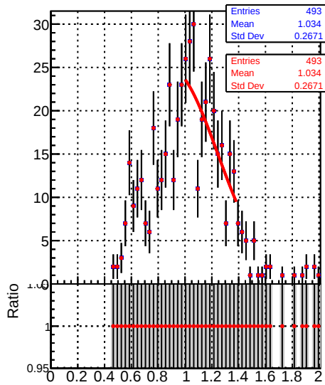
Raw Jet response (pT/pTgen) in 15 \leq p_t < 21, 0.5 \leq |\eta| < 1.3
