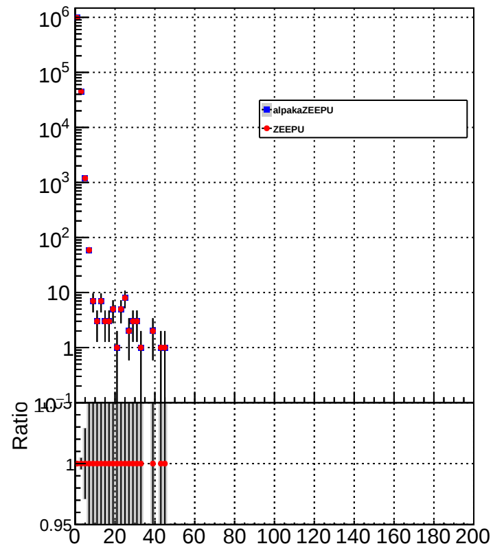
HF_EM_particlePtMid
