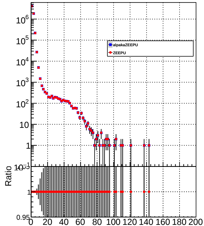
HF_hadronPtMid
