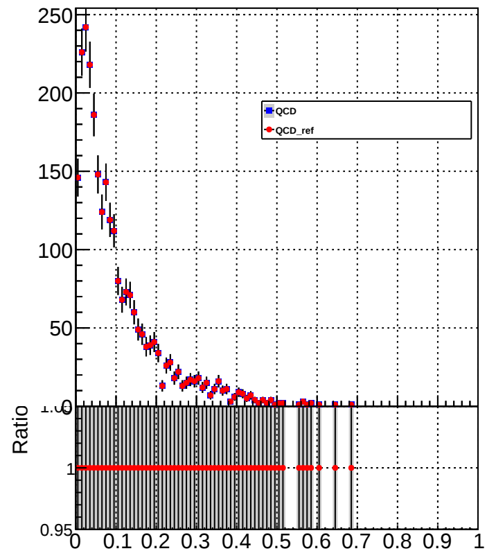
HFHadronEtFraction
