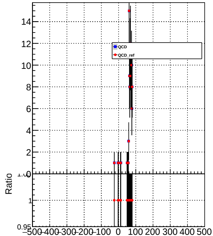
METResolution_GenMETTrue_MET60to80
