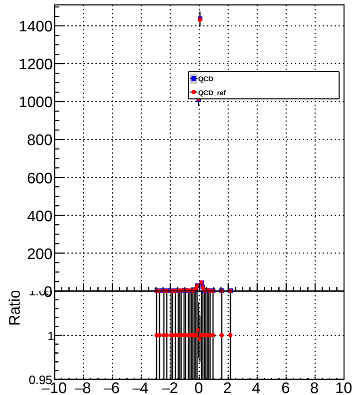
METUnc_ElectronEnUp
