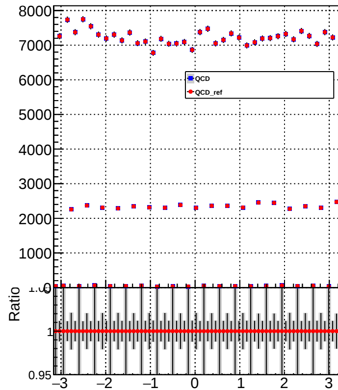
HF_EM_particlePhi
