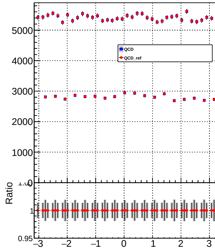
HF_hadronPhi
