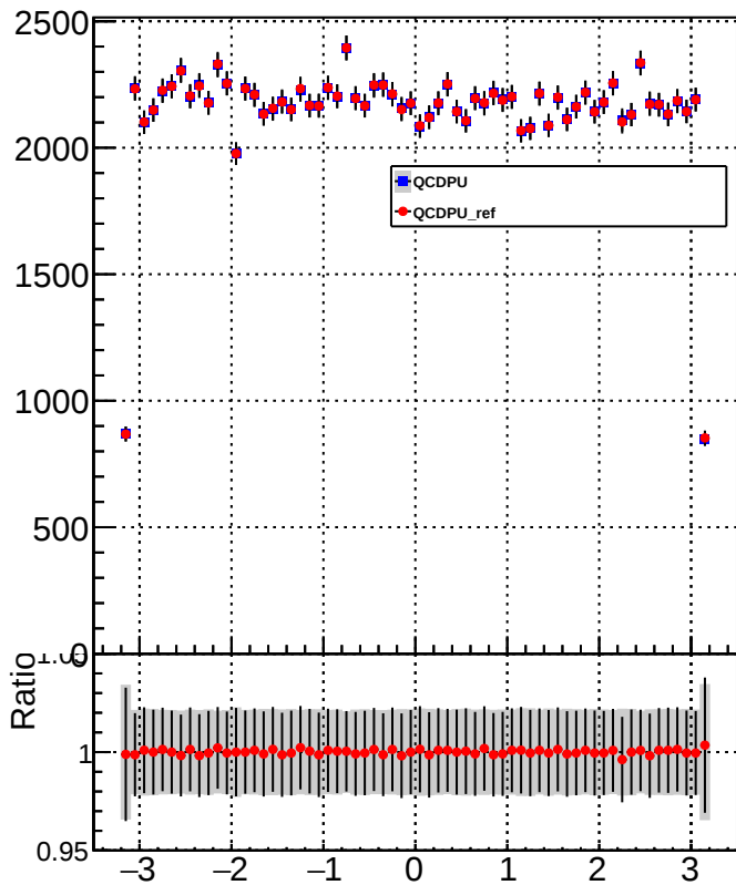
CorrJetPhi Pt>40
