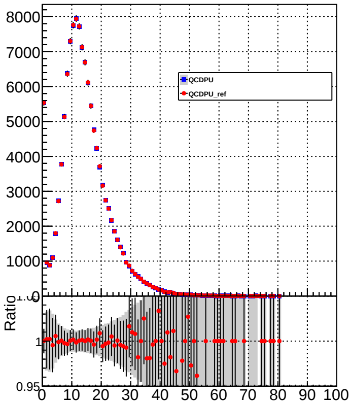
chargedMultiplicity
