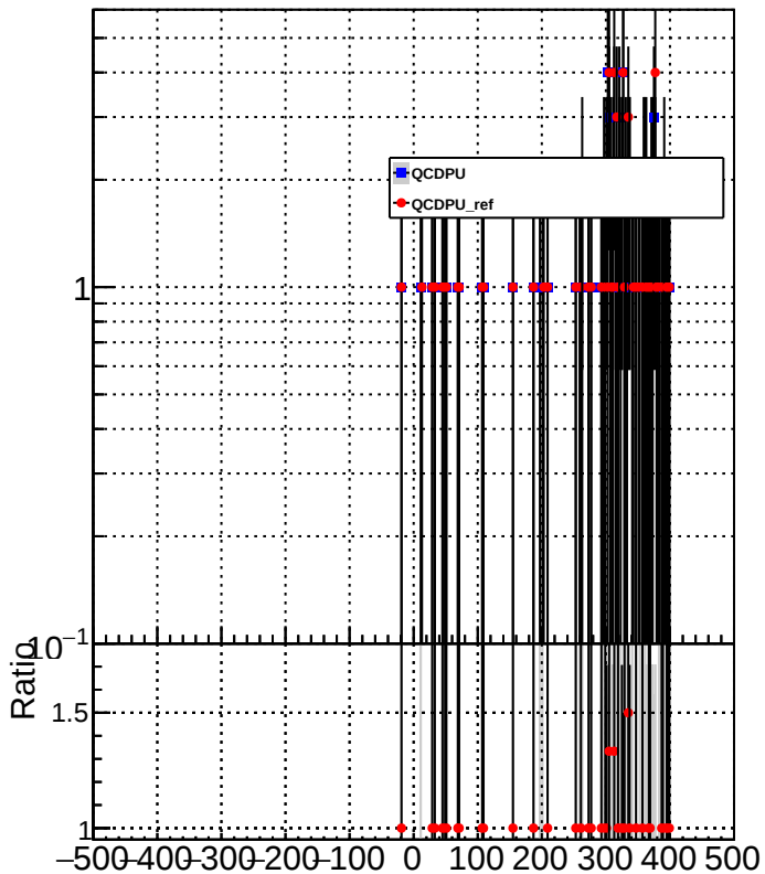
METResolution_GenMETTrue_MET300to400
