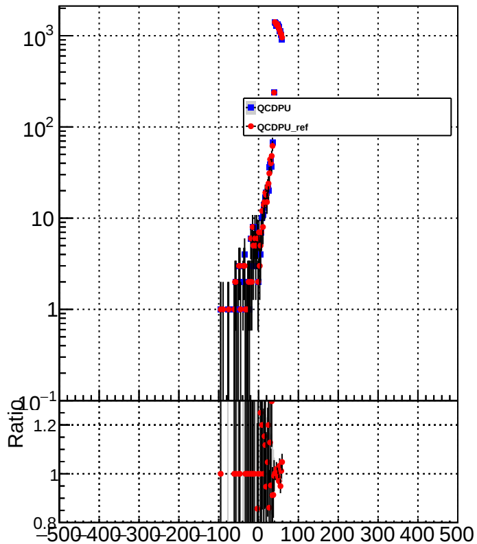
METResolution_GenMETTrue_MET40to60
