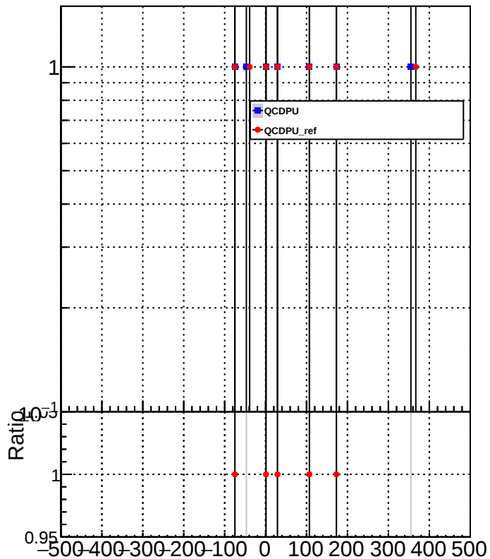
METResolution_GenMETTrue_MET500
