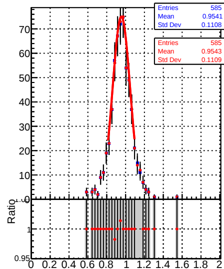
Raw Jet response ( p_T/p_{T\text{gen}} ) in 196 \leq p_T < 272 , 2.5 \leq |\eta| < 3.0
