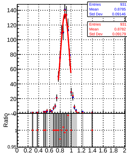
Raw Jet response ( p_T/p_{T\text{gen}} ) in 196 \leq p_T < 272 , 2.1 \leq |\eta| < 2.5
