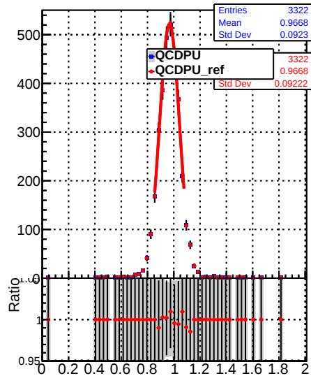
Raw Jet response ( p_T/p_{T\text{gen}} ) in 196 \leq p_T < 272 , 0.0 \leq |\eta| < 0.5
