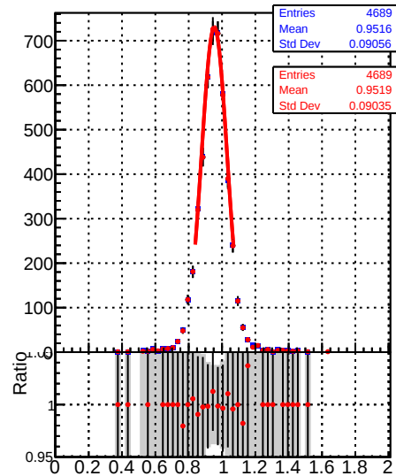
Raw Jet response ( p_T/p_{T\text{gen}} ) in 196 \leq p_T < 272 , 0.5 \leq |\eta| < 1.3
