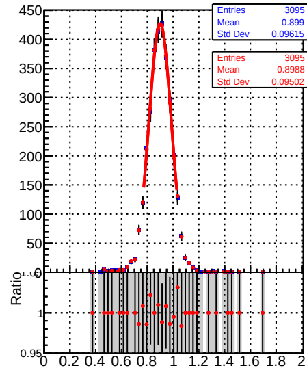
Raw Jet response ( p_T/p_{T\text{gen}} ) in 196 \leq p_T < 272 , 1.3 \leq |\eta| < 2.1
