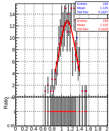
Raw Jet response ( p_T/p_{T\text{gen}} ) in 196 \leq p_T < 272 , 3.0 \leq |\eta| < 5.0
