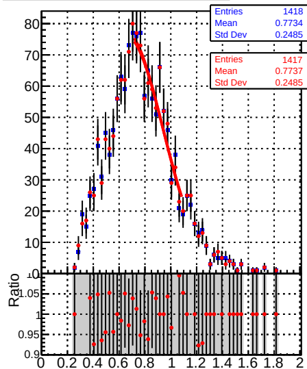
Raw Jet response (pT/pTgen) in 21 &lt;= pt &lt; 28, 2.1 &lt;= |eta| &lt; 2.5
