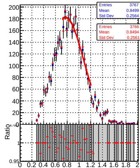
Raw Jet response (pT/pTgen) in 21 &lt;= pt &lt; 28, 1.3 &lt;= |eta| &lt; 2.1
