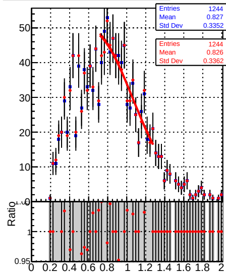
Raw Jet response (pT/pTgen) in 21 &lt;= pt &lt; 28, 2.5 &lt;= |eta| &lt; 3.0
