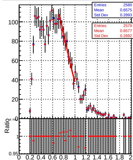
Raw Jet response (pT/pTgen) in 21 &lt;= pt &lt; 28, 3.0 &lt;= |eta| &lt; 5.0
