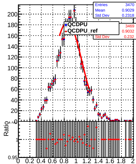
Raw Jet response (pT/pTgen) in 21 &lt;= pt &lt; 28, 0.0 &lt;= |eta| &lt; 0.5
