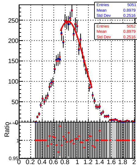
Raw Jet response (pT/pTgen) in 21 &lt;= pt &lt; 28, 0.5 &lt;= |eta| &lt; 1.3
