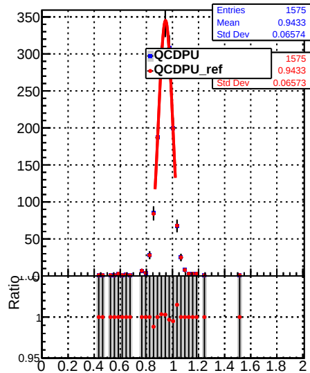
Raw Jet response (pT/pTgen) in 548 &lt;= pt &lt; 686, 0.0 &lt;= |eta| &lt; 2.5
