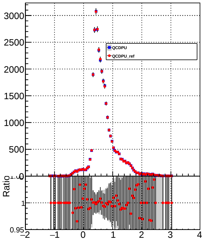
electronLog10Pt
