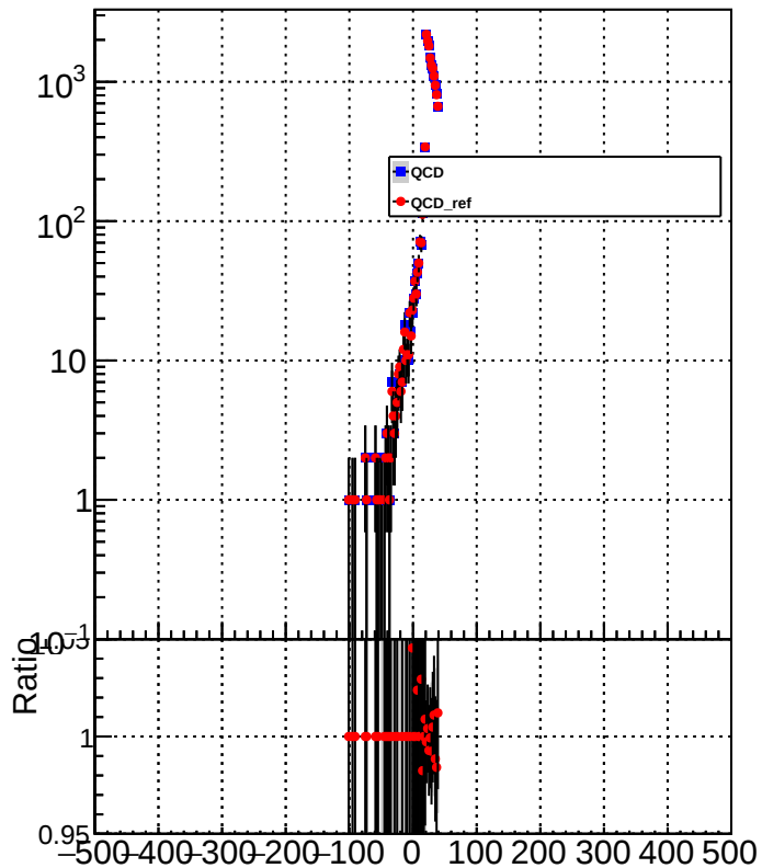
METResolution_GenMETTrue_MET20to40
