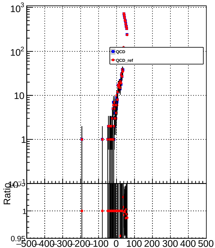
METResolution_GenMETTrue_MET40to60
